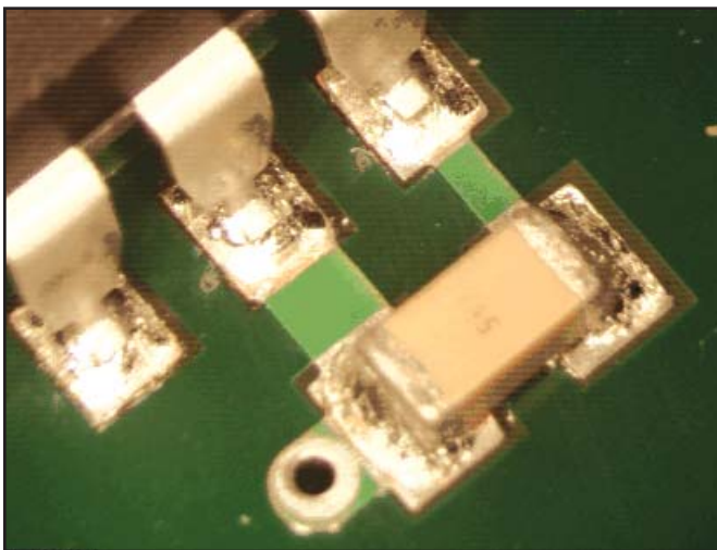
Figure 3C: Cold Solder
